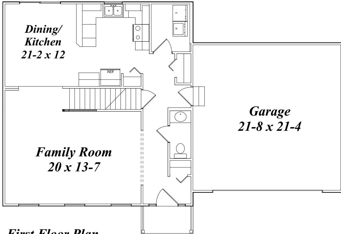
First Floor Plan 840 Square Feet
