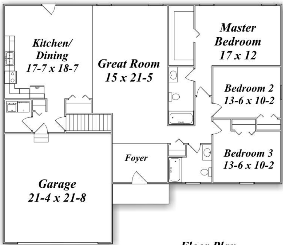
Floor Plan 1800 Sq Ft
